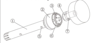
Work head disassembly scheme
